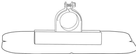
Small Pipe Diameter Securement
