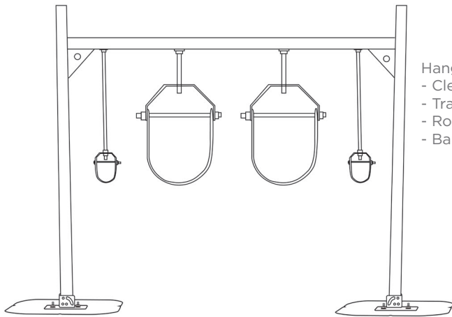
Attached M.E.P Frame Securement
